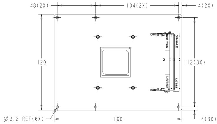
Figure 2 OCM PCBA Top View
