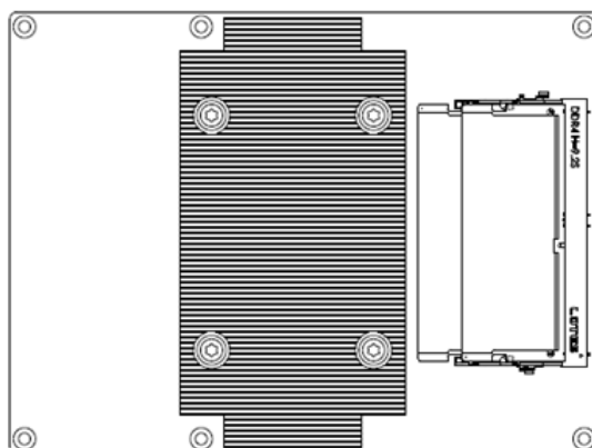
Figure 5 OCM Wireframe View-Top
