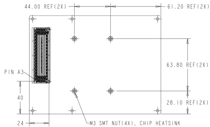
Figure 4 OCM PCBA Bottom View
