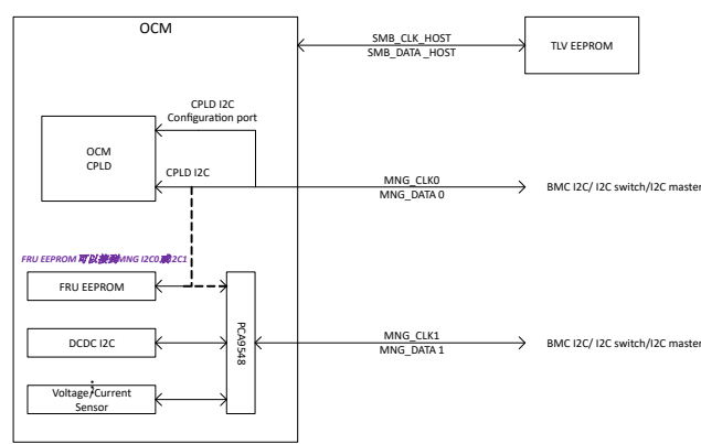
Figure 12 I2C 信号处理逻辑
