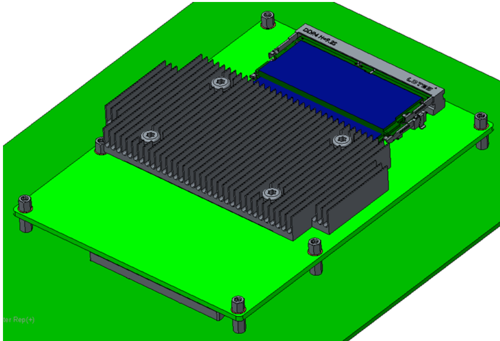
Figure 1 Open Control Module Isometric View
