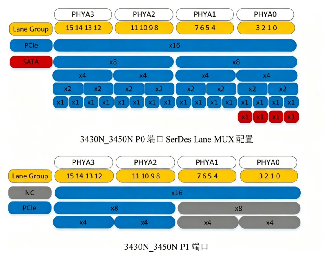
Figure 17 3430N/3450N PCIE 配置
