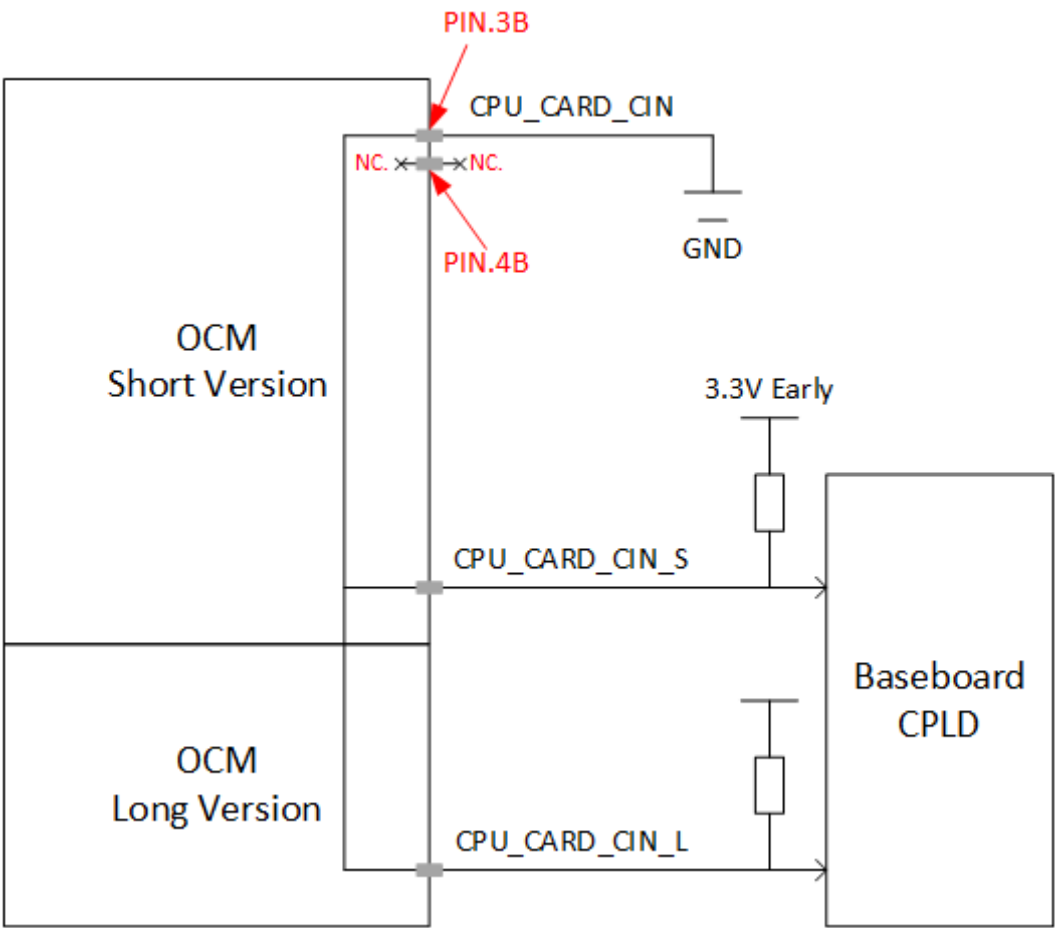
Figure 15 Present 信号处理逻辑
